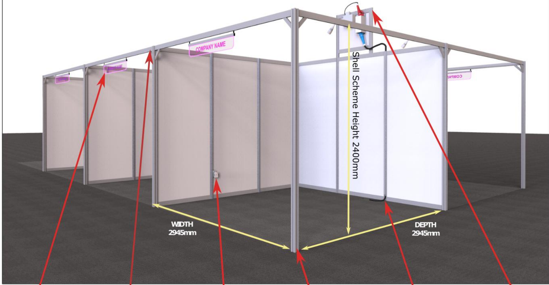
LED NAMEBOARD
